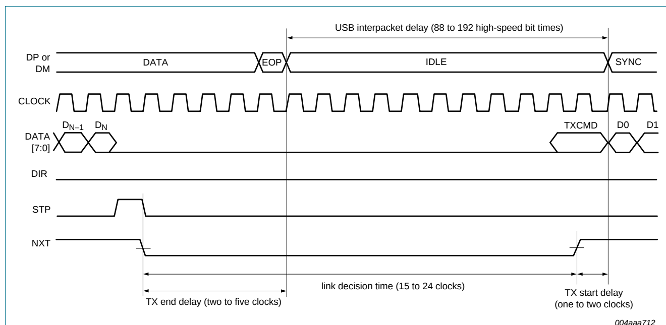
Fig 15. High-speed transmit-to-transmit packet timing
