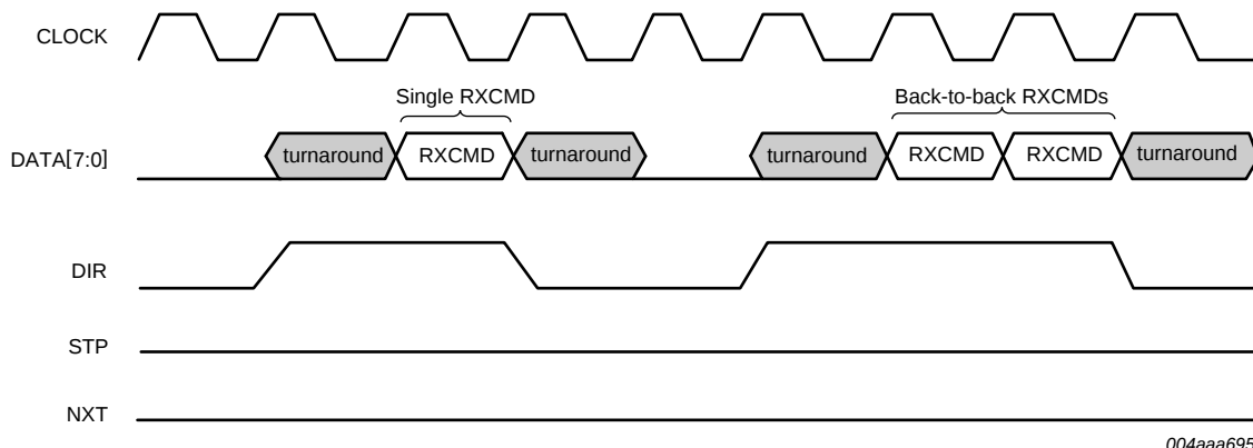
Fig 10. Single and back-to-back RXCMDs from the SAF1508BET to the link
